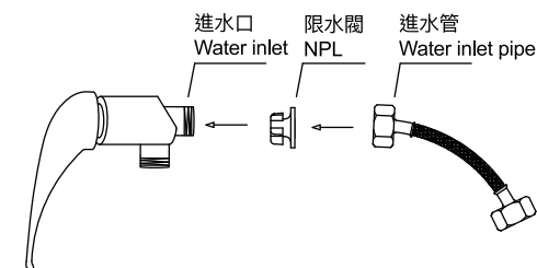
NPL Installation Diagram
